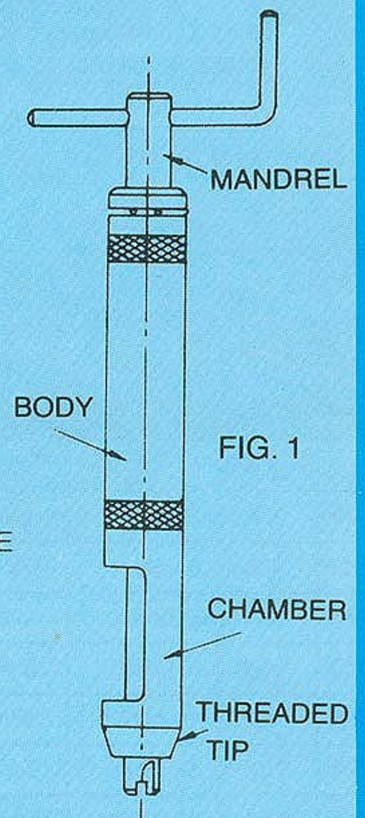
PREWINDER TYPE INSERTING TOOL
